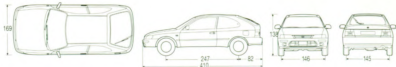
Hatchback 3-drs
