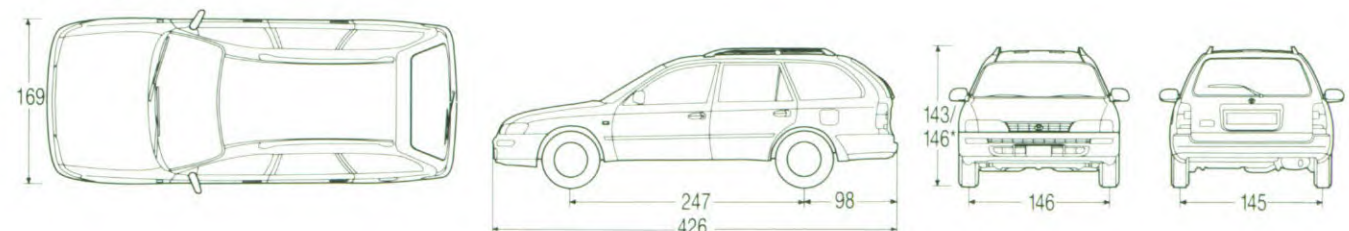
Stationwagon
