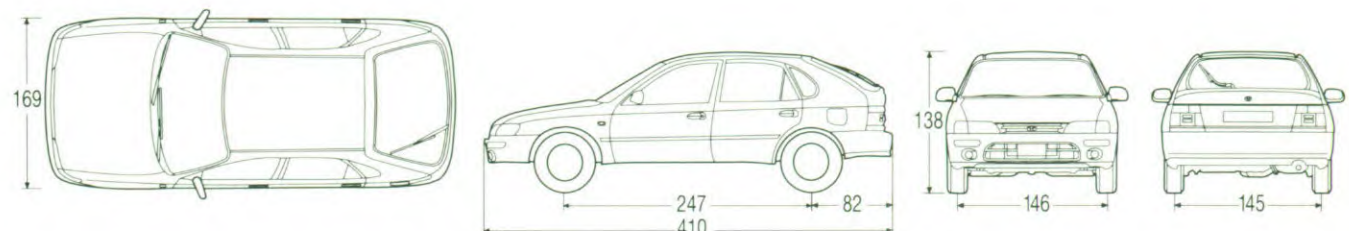
Hatchback 5-drs
