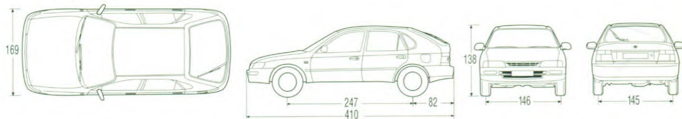
Hatchback 5-drs
