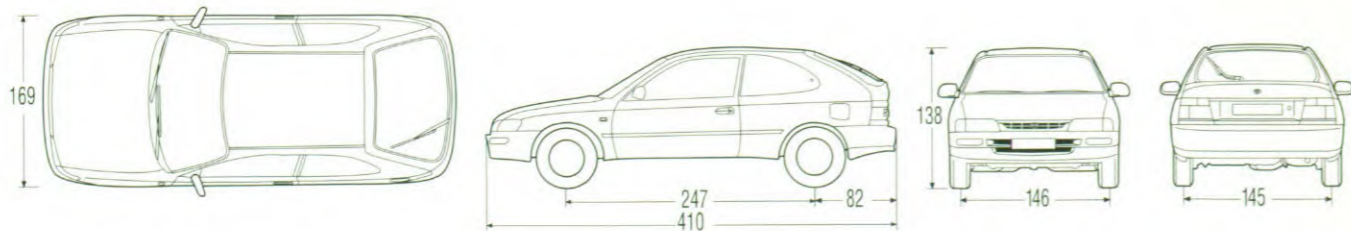
Hatchback 3-drs
