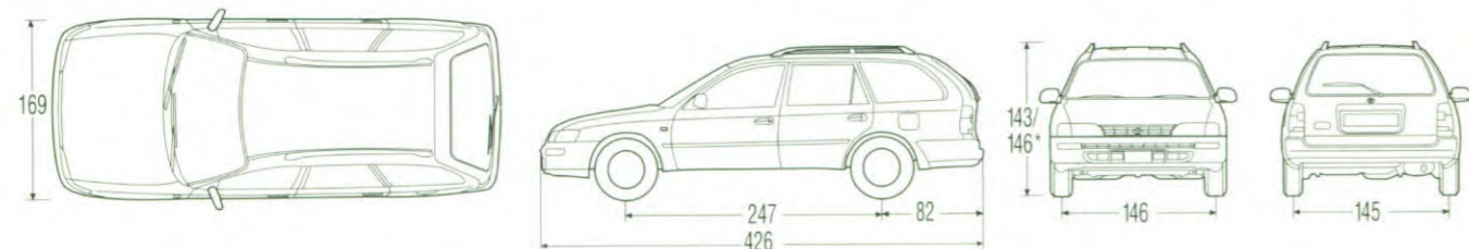
Stationwagon
