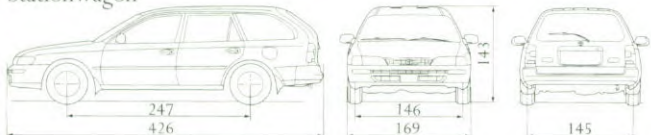
Stationwagon
