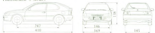
Hatchback 3-deurs
