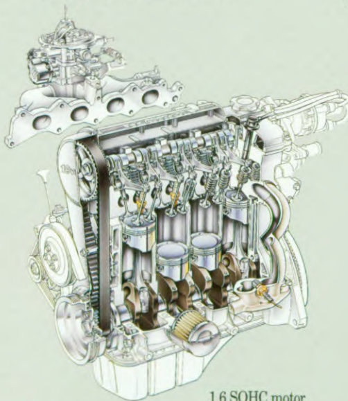
1.6 SOHC motor
