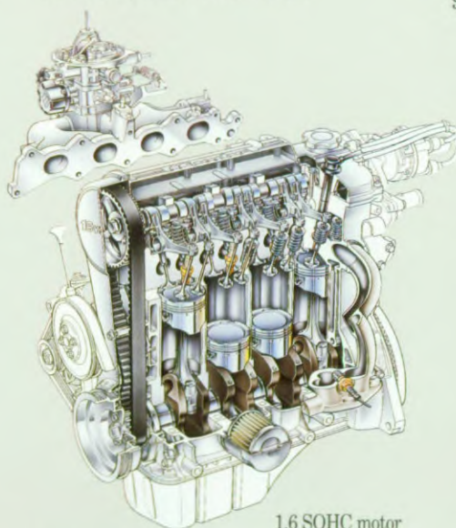
1.6 SOHC motor
