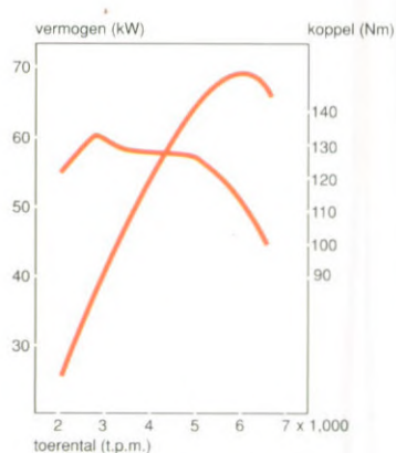
G16B motor prestatie-curves
