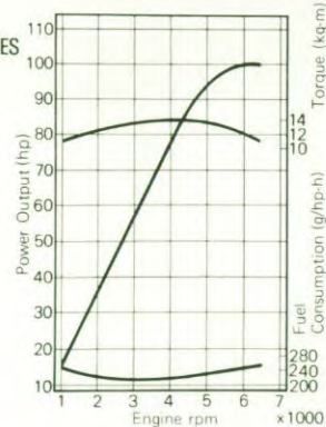
2000ccENGINE PERFORMANCE CURVES
