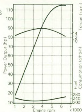
2000ccENGINE PERFORMANCE CURVES
