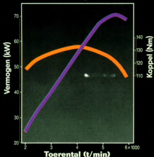
• G16B vermogens curve
