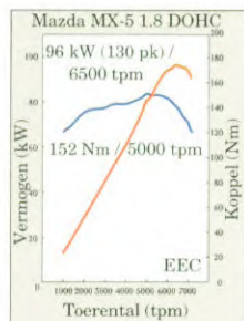
Prestatiecurves 1,8-liter motor (ECE)
