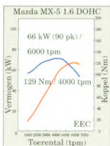
Prestatiecurves 1,6-liter motor (ECE)
