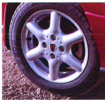
Alloy Wheel (6 Spoke) RRC 108940 MNH Centre Cap DTC 10054 MNH Wheel Nut RRD 100310 Wheel Dimension 5.5J x 14
