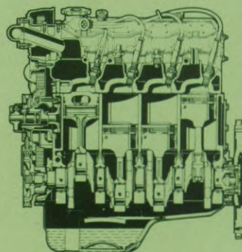
1600 TC motor
