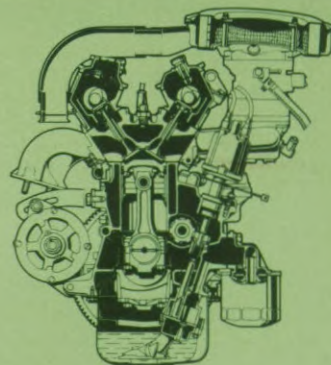
1600 TC motor
