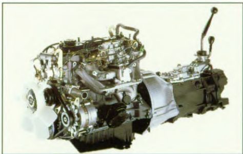
De 2-liter benzinemotor.
