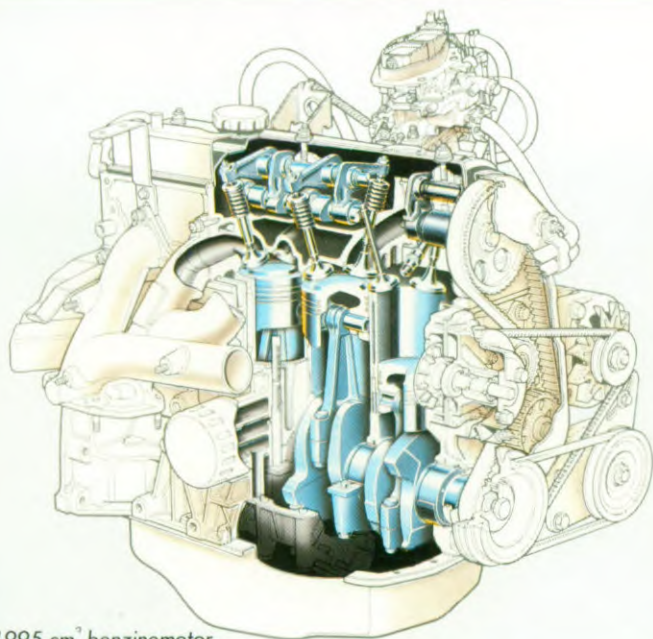
1995 cm 3 benzinemotor
