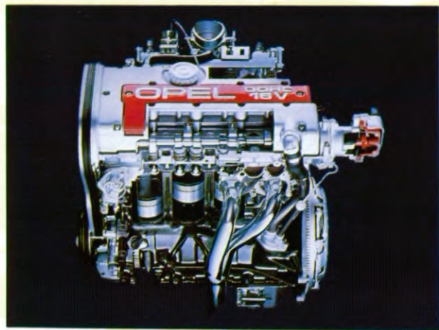
2-liter 16-kleppenmotor, 110 kW (150 DIN-ph).
