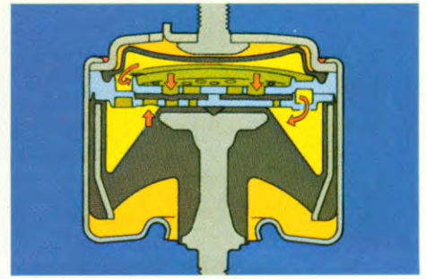
Hydro-elastische motorophanging.
