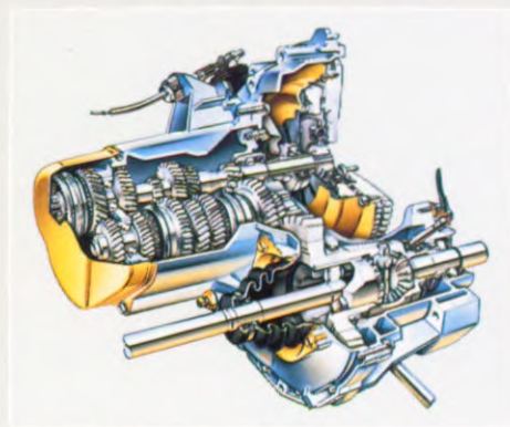
Compacte krachtoverbrenging.
